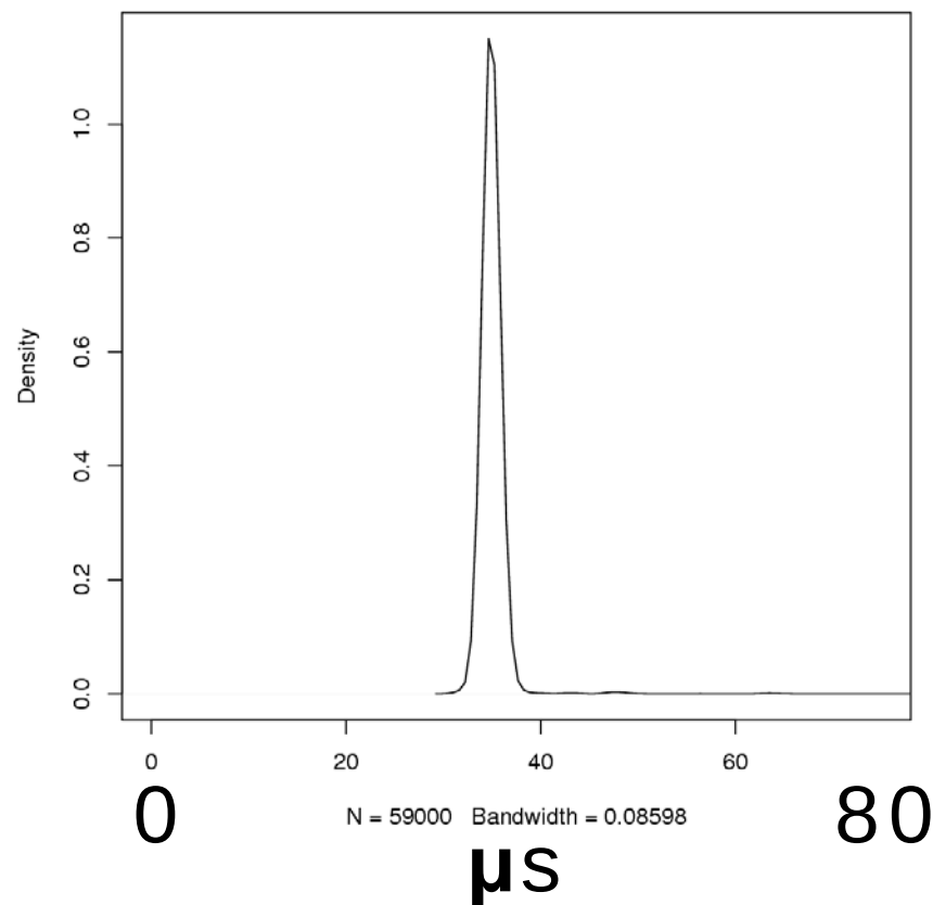
DAG offset density, standard testbox
