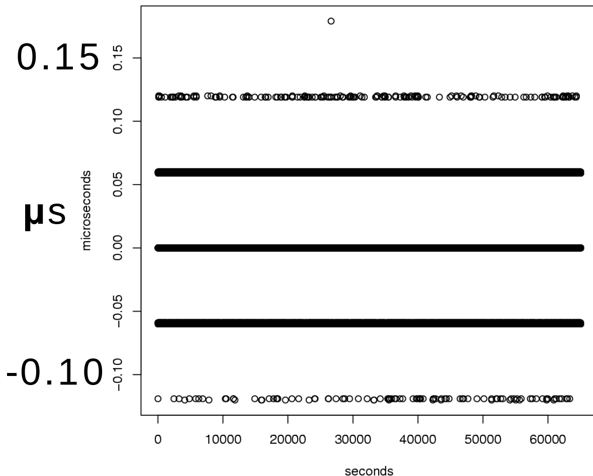
Two DAG cards cross-connected: offset plot
