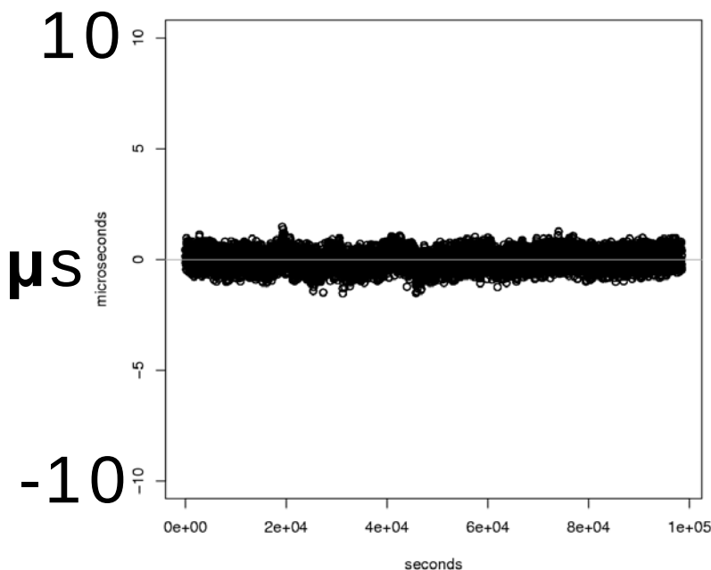
PPS offset plot - NTP PPS
